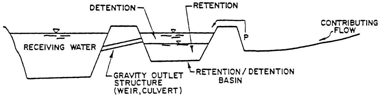
Figure 2.5-3 Pumped flow tailwater example.
