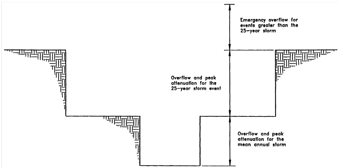
Figure 4.5-1 Conceptual design of a multi-stage outlet structure.
