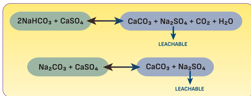
Bicarbonate ( 2\text{NaHCO}_3 ) and carbonate ( \text{Na}_2\text{CO}_3 ) reductions following gypsum ( \text{CaSO}_4 ) application.
