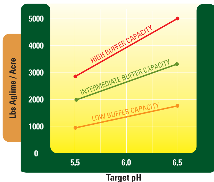
FIGURE 5.18: Effects of buffering capacity on lime requirements
