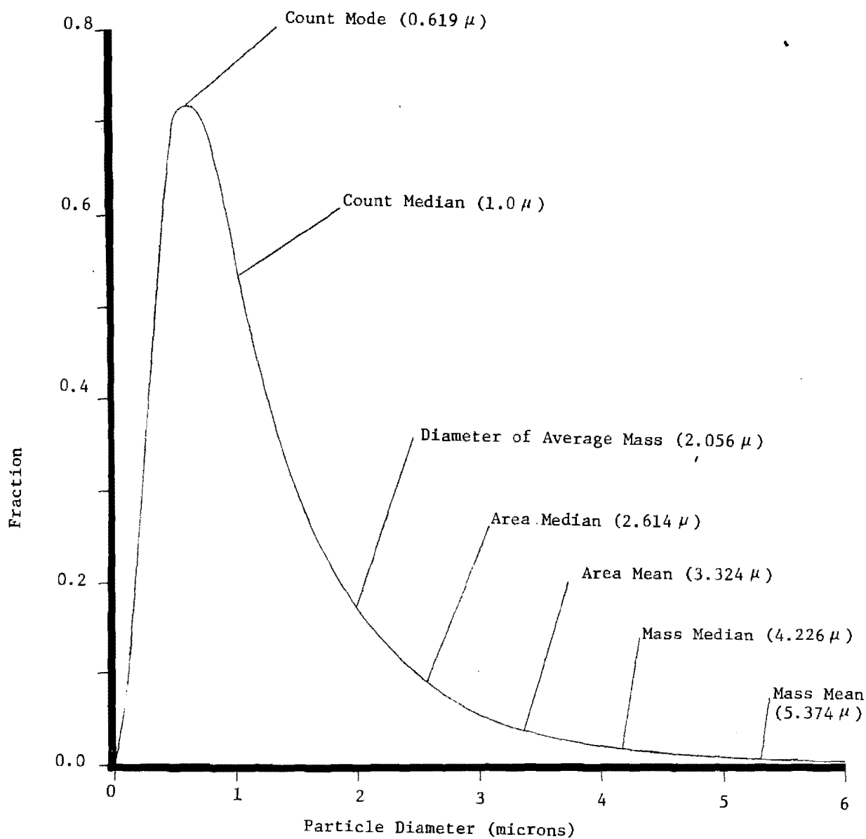
Figure 9.1: TYPICAL SIZE DISTRIBUTION OF PARTICLES IN THE ATMOSPHERE SHOWING VARIOUS AVERAGE DIAMETERS (VOLZ, 1959)
