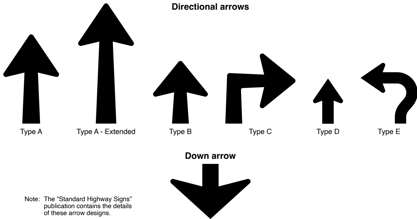
Figure 2D-3. Arrows for Use on Guide Signs
