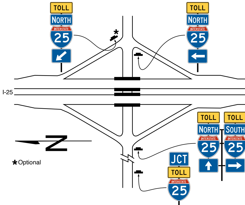
Figure 2F-5. Example of Minor Interchange Crossroad Signing for an Approach to a Toll Highway
