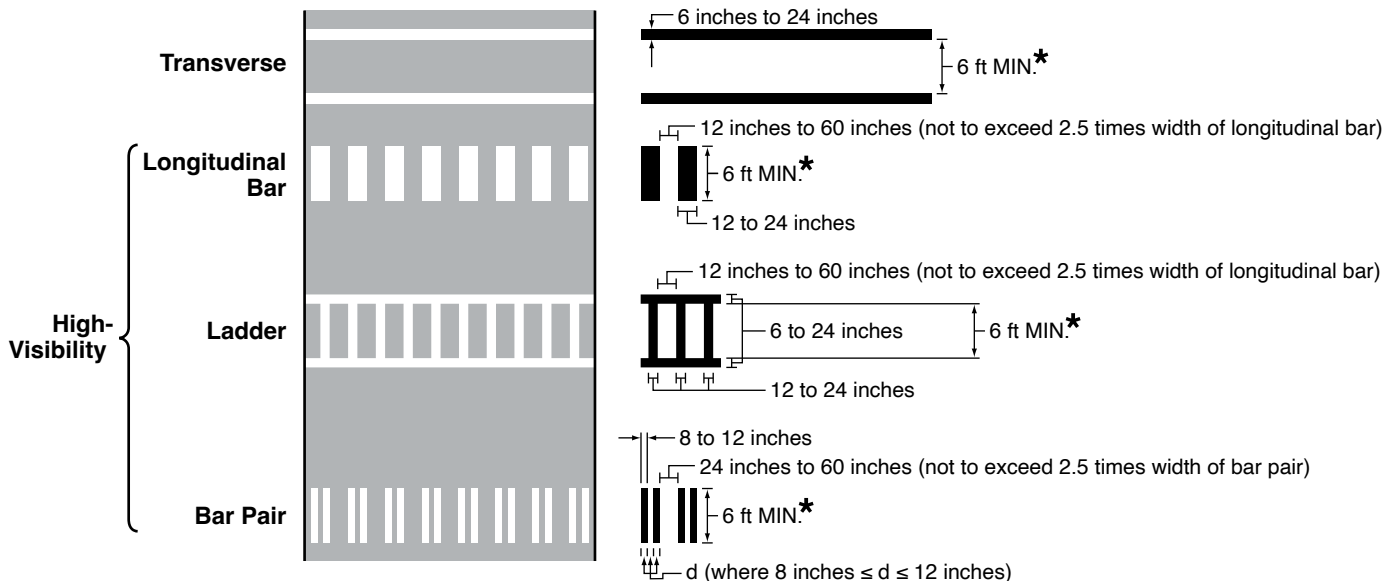
Figure 3C-1. Crosswalk Markings
