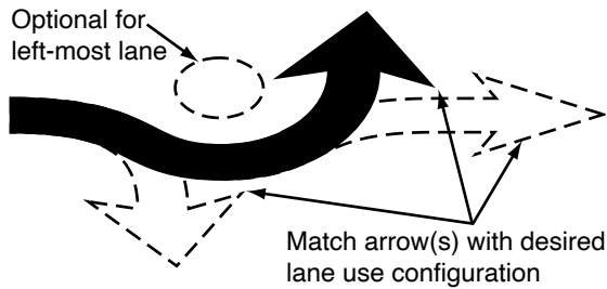
F – Curved-stem lane-use arrows
