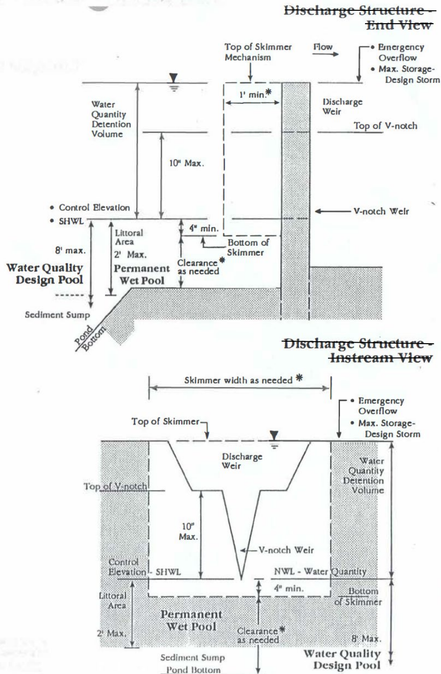
FIGURE 1 Conservation Wet Detention Discharge Structure End View and Discharge Structure Instream View
