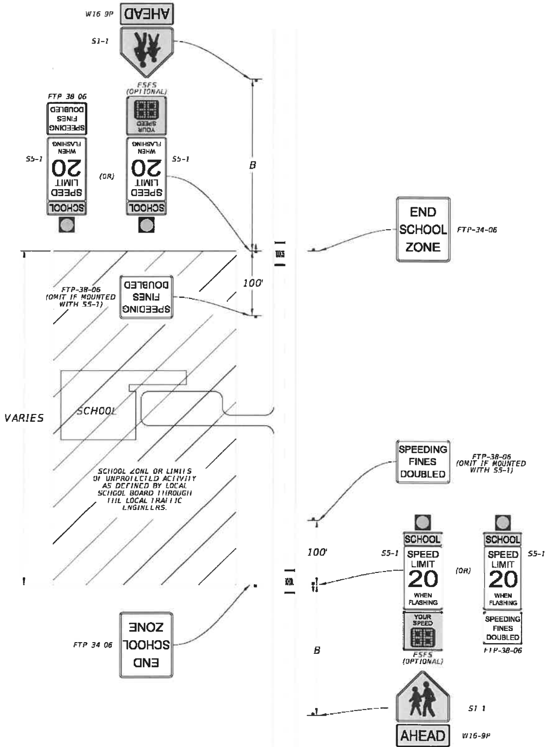
Figure 15-13 Typical School Zone Fronting the School Property Without a School Crossing
