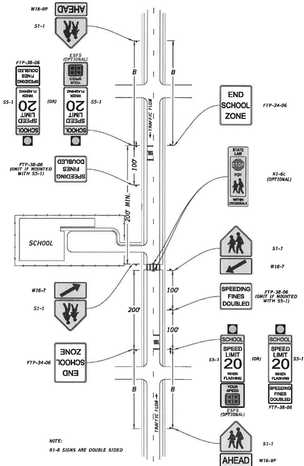
Figure 15-12 Typical School Zone With School Crossing (2- or 3-Lane, 2-Way) (40 mph or less) Mid-block or on Thru Street at an Intersection
