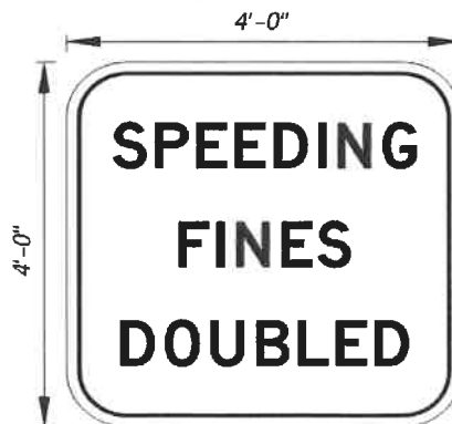
Figure 15-7B Speeding Fines Doubled Sign (Overhead Option – FTP 39-06)
