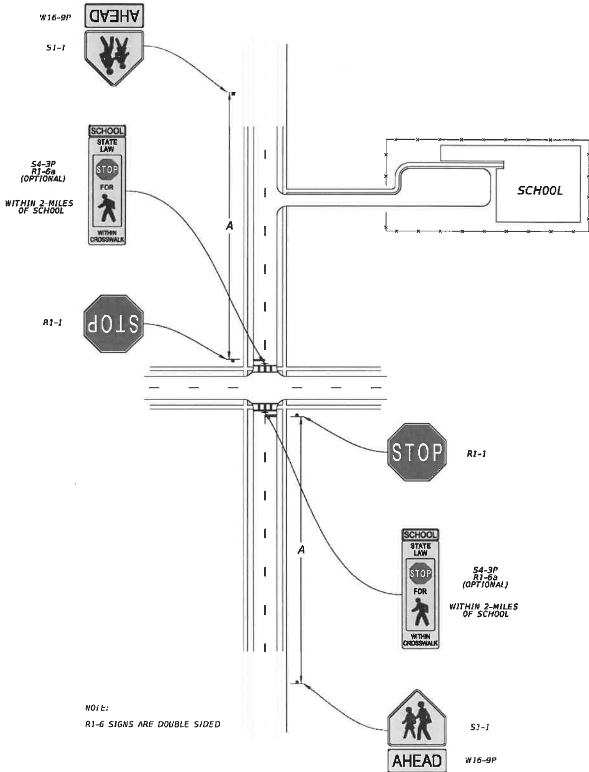
Figure 15-4 School Crosswalks at a Stop Controlled Intersection Without a School Zone
