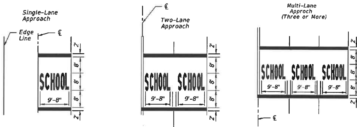
Figure 15-15B School Pavement Message Layouts for Single and Multi-Lane Approaches
