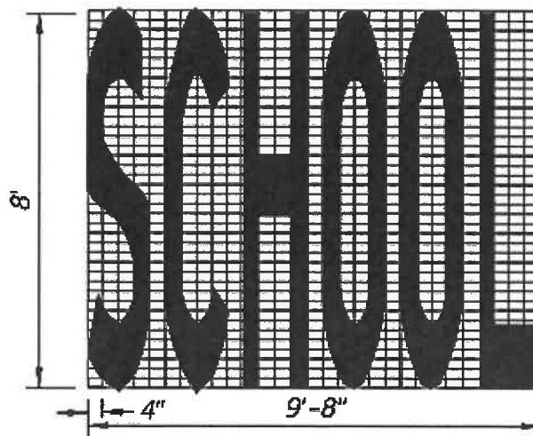
Figure 15-15A. School Pavement Message Details
