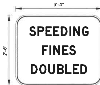
Figure 15-7A Speeding Fines Doubled Sign (Ground-Mounted Option – FTP 38-06)
